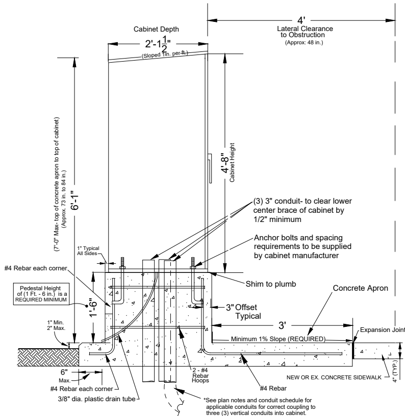
SIDE VIEW (Door & Apron to the Right)
