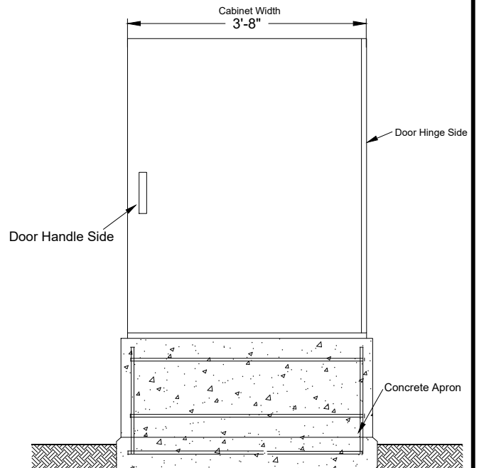
FRONT VIEW (Door Side) (All dims other than width shown on SIDE VIEW)
