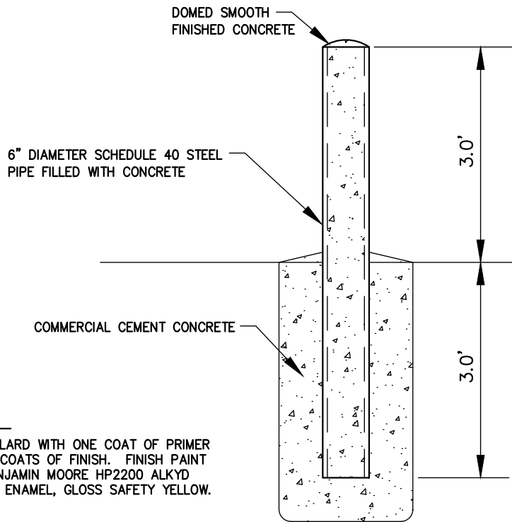
BOLLARD SECTION A-A
