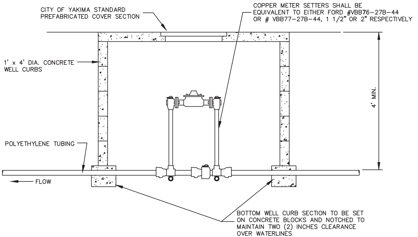
W10 1 1/2" & 2" METER INSTALLATION NTS City of Yakima - Engineering Division
