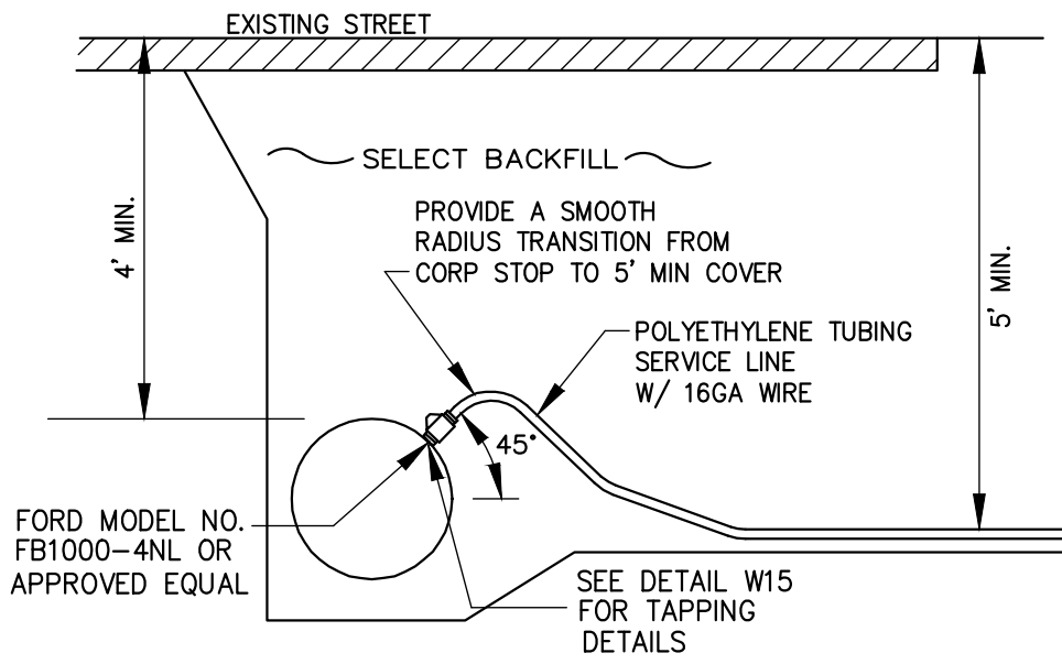
SERVICE LINE W/O METER DETAIL
