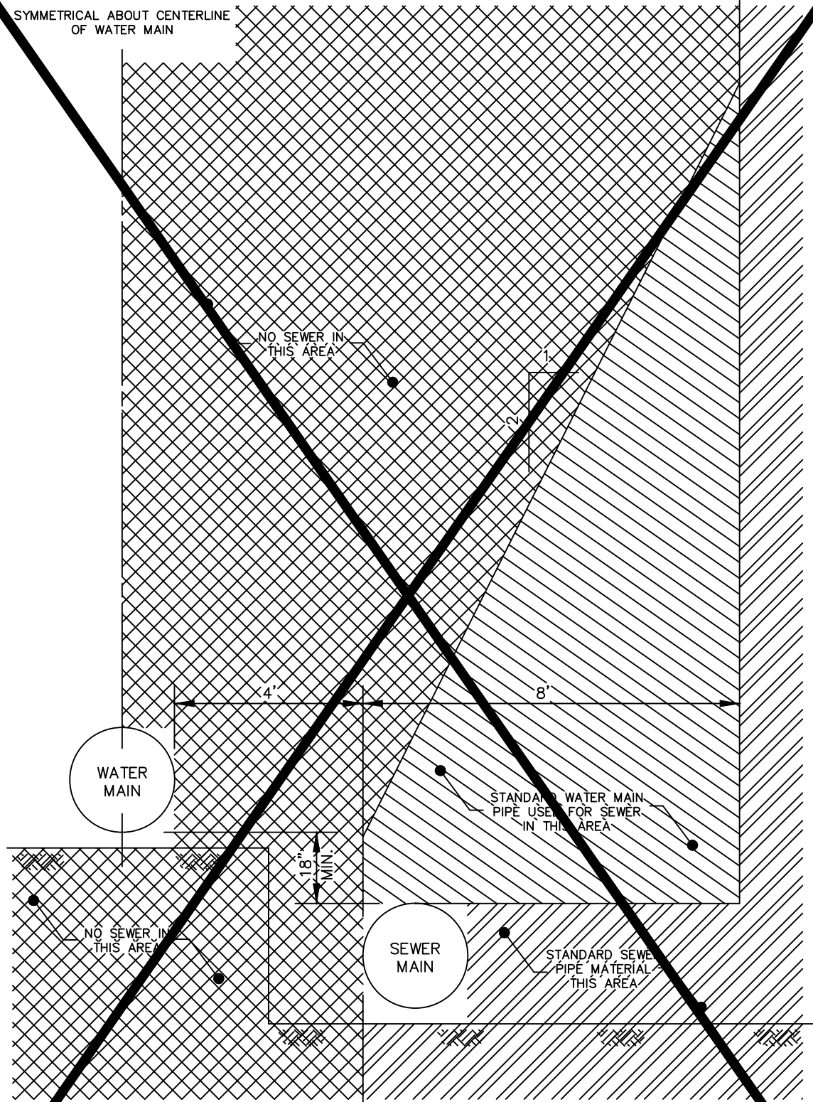
W16 PARALLEL WATER/SEWER SEPARATION NTS City of Yakima - Engineering Division
