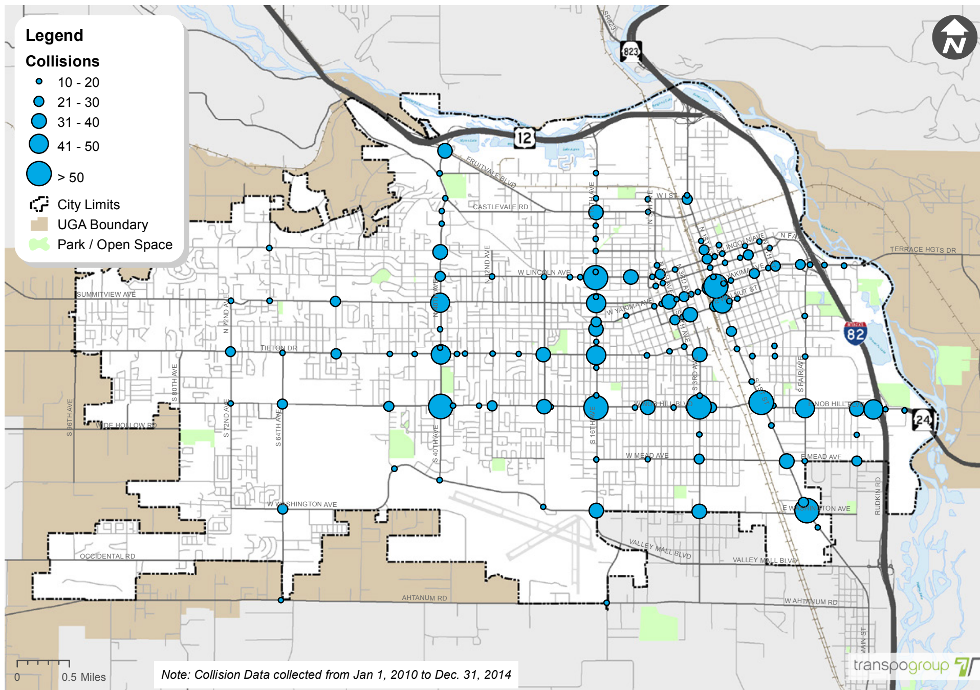
Figure 2-11. Vehicle Collisions (2010 – 2014)
